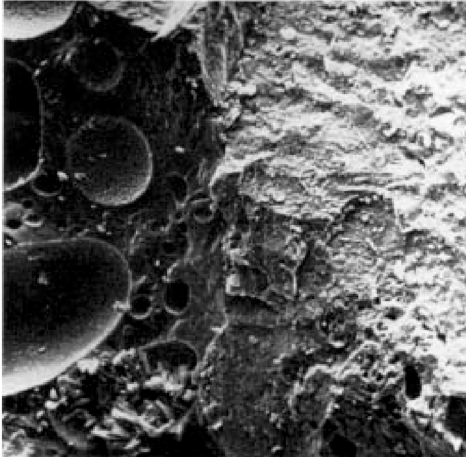
Figure 22. Fractured surface of concrete from USS Selma . (Expanded aggregate is on the left, and the cement paste is on the right. Micrograph width is 550 \mu\text{m} ) (from Bremner, Holm, and Morgan 1996, with permission of ACI)
