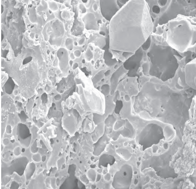
Figure 2 Cellular Pore Structure ESCS Media
